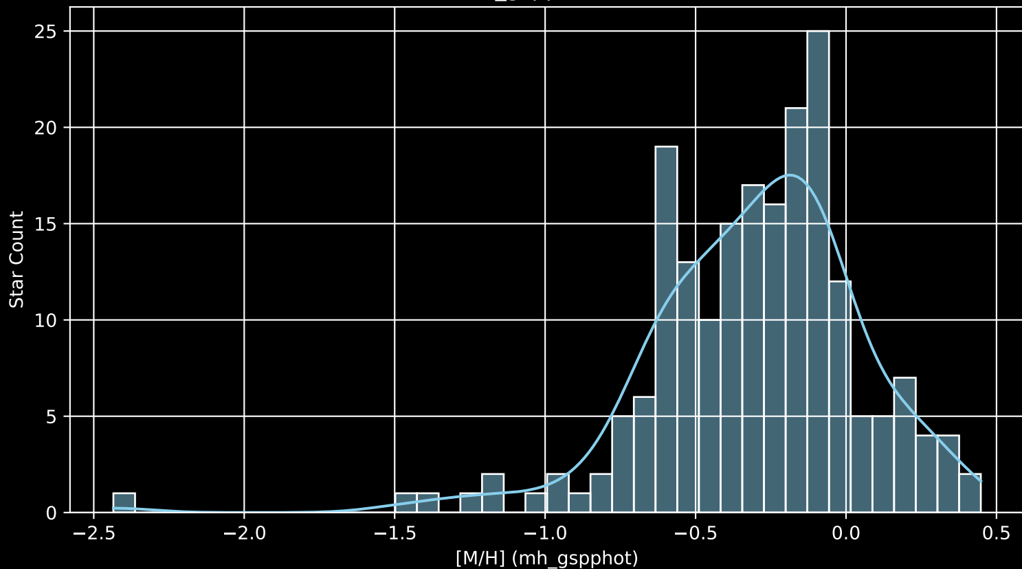
APOGEE DR17 Field: [335+61_btx [M/H] (mh_gspphot) (n= 198)
