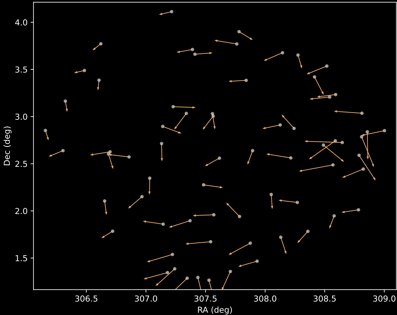
APOGEE DR17 Cluster 3 Proper Motion Vectors (n=67)
