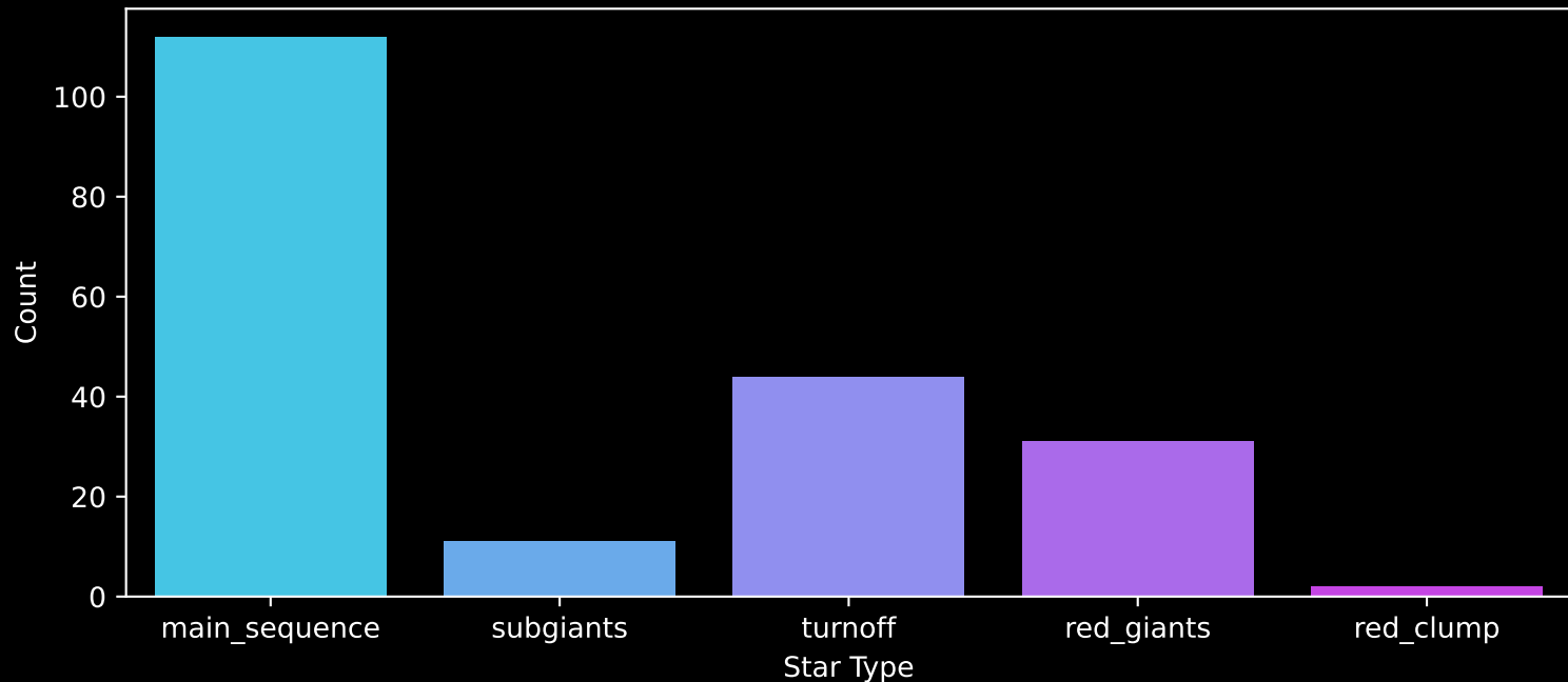
APOGEE DR17 Field: [335+61_btx] Count plot of Star Type
