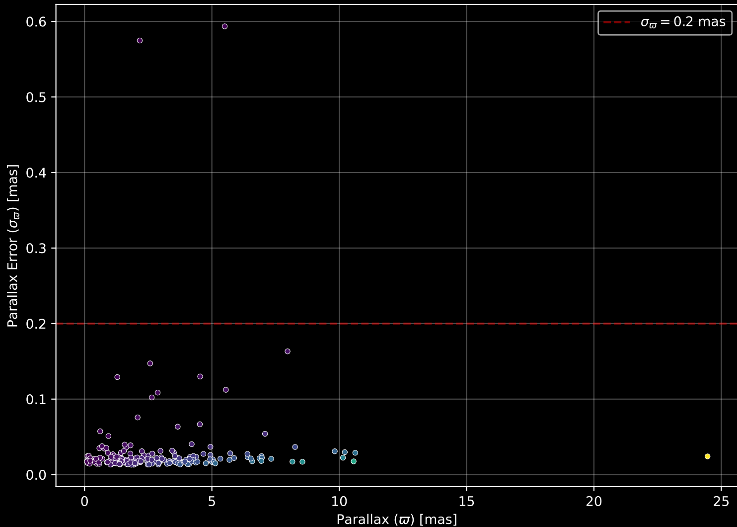
APOGEE DR17 Field: [335+61_btx] Parallax Quality (n= 200)
