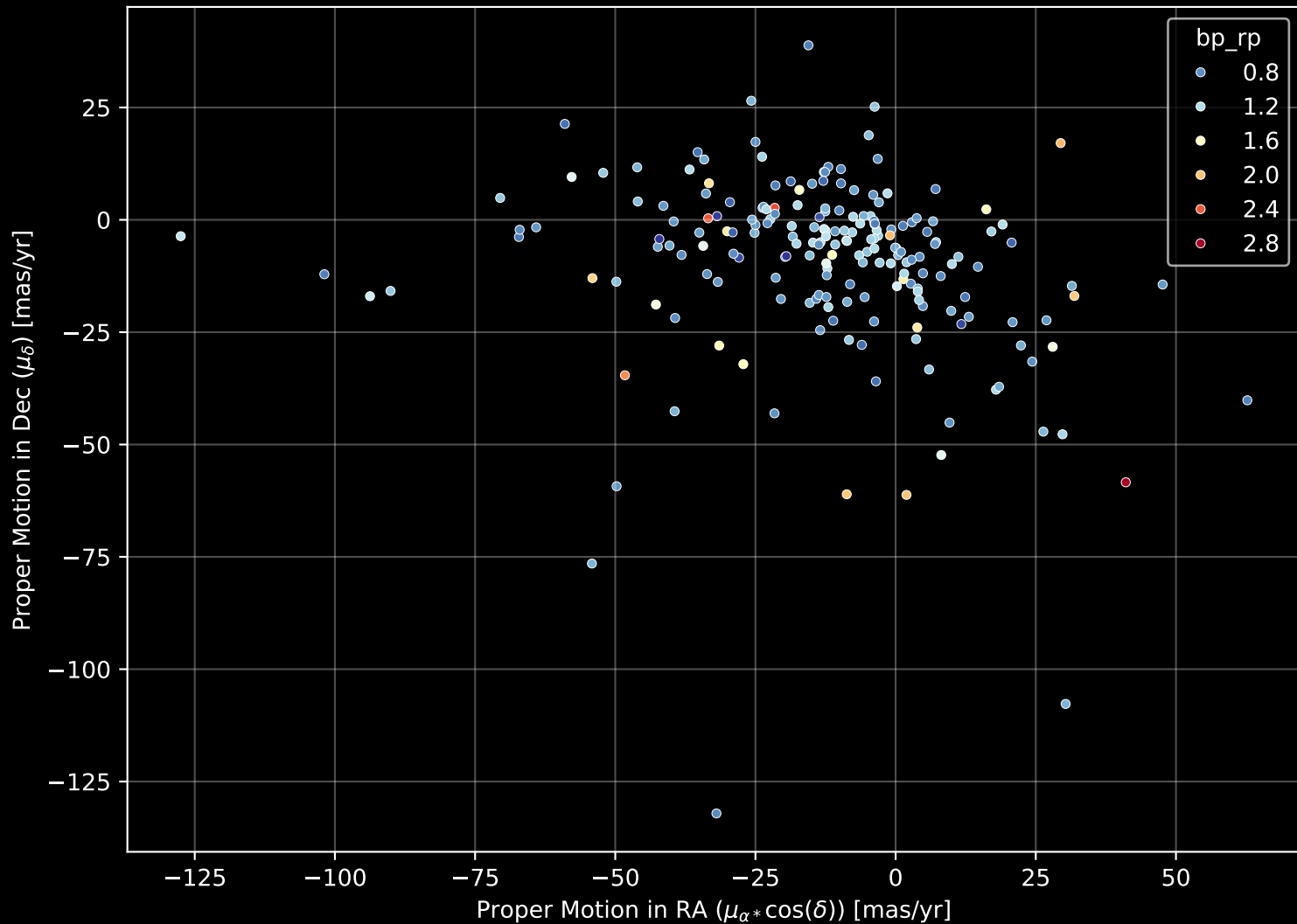
APOGEE DR17 Field: [335+61_btx] Proper Motion Diagram (n= 200)
