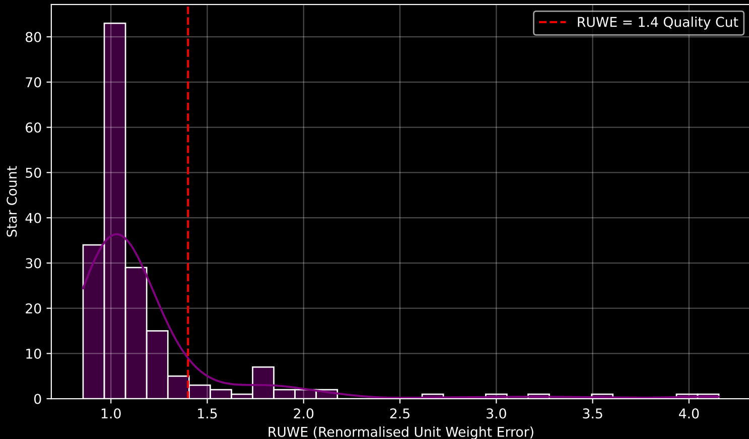
GAPOGEE DR17 Field [335+61_btx] RUWE Distribution (n= 191)
